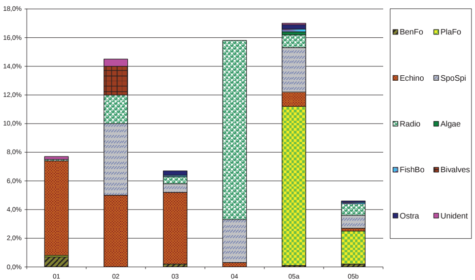
Chart 2 - Petrographic fossil distribution in chert microfacies from Peștera Valley; Legend: Unident – Unidentified fossils; Ostra – Ostracodes; Bivalves – fragments of bivalve shells; FishBo – fragments of fish bones; Algae – fragments and fragmented parts of calcareous algae; Radio – Radiolarians; SpoSpi – Sponge spicules; Echino – fragments of echinoderms; PlaFo – planktonic foraminifera; BenFo – benthic foraminifera.
