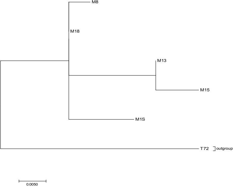
Fig. 3: Molecular Phylogenetic analysis by Maximum Likelihood method For inferring the evolutionary history of the analysed human bone samples, we have used the Maximum Likelihood method based on the Tamura-Nei
